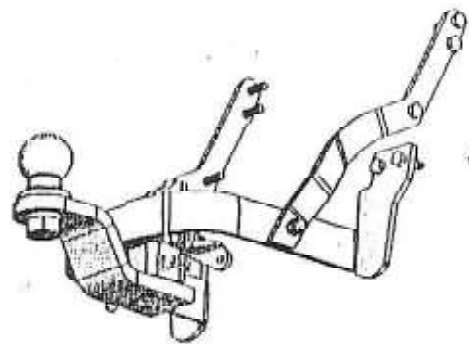
ASSEMBLED VIEW 5/16" x 1" LONG BOLT,
